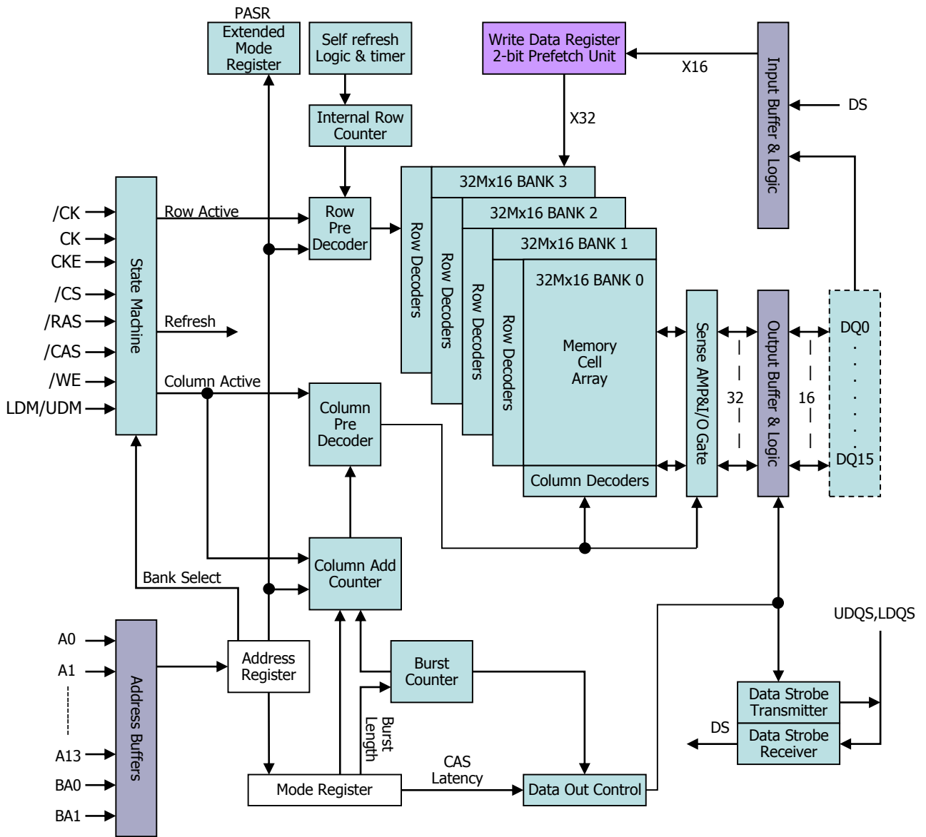
Figure 2.1 : Functional Block Diagram (128Mb X 16)
