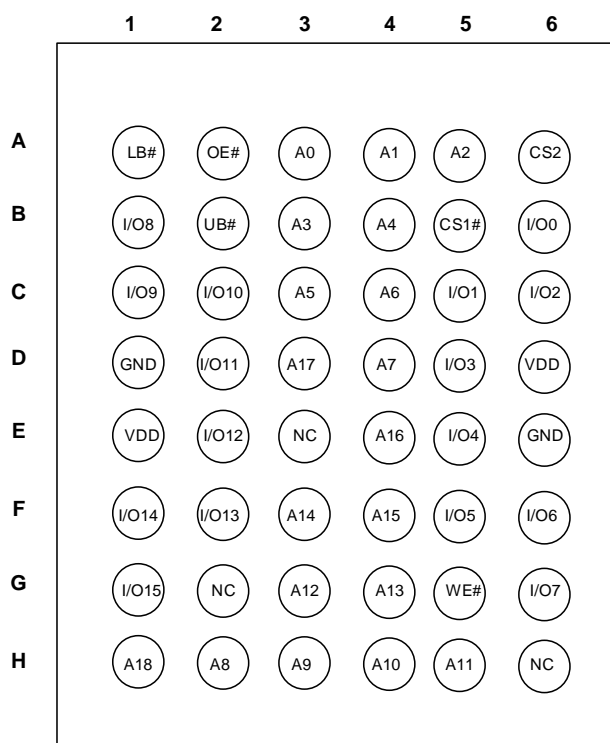
48-Pin TSOP (TYPE I), 2 CS
