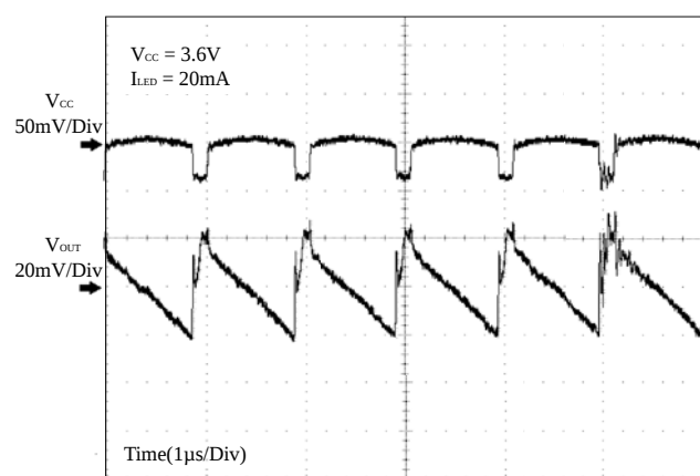
Figure 9 Ripple Voltage
