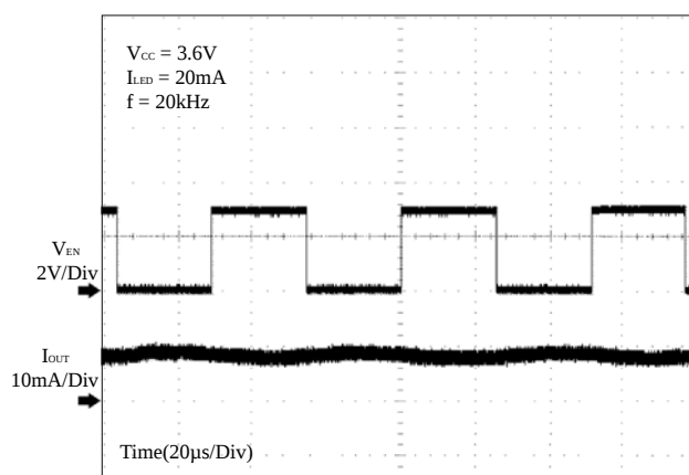
Figure 10 PWM Dimming from EN
