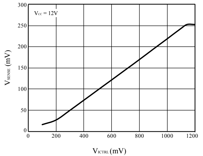
Figure 17 V_{SENSE} vs. V_{CTRL}
