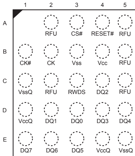
Figure 16.2 24-ball BGA, 5x5 Ball Footprint (FAE024), Top View
