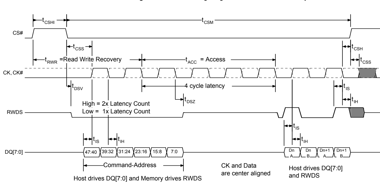
Figure 8.7 Write Timing Diagram - No Additional Latency
